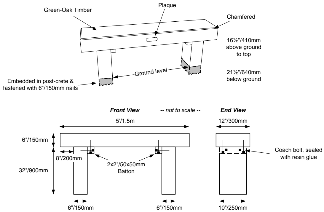
Bench Plan
